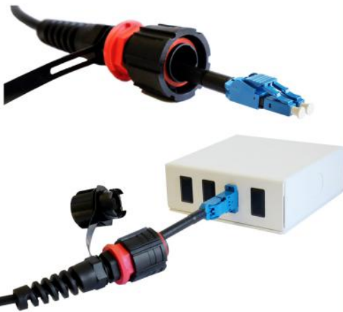
DIRECT CONNECTION TO LC ADAPTERS OR SFP'S
